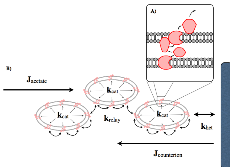
Figure 1 A) Cartoon showing possible paths of electron transfer across the inner and outer membranes of an electroactive bacterium. B) Schematic representation of mass transfer and kinetic limitations in an electrode-reducing biofilm in the absence of any soluble redox-active compounds. The total current is a function of: acetate flux ( J_{\text{acetate}} ), irreversible metabolic reactions supplying electrons to the membrane ( k_{\text{cat}} ), electron transfer around and between cells, relaying electrons to the interfacial contact point ( k_{\text{relay}} ), interfacial transfer by proteins actually in contact with the electrode ( k_{\text{het}} ), and counterion flux from the film ( J_{\text{counterion}} ).
