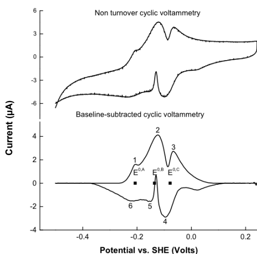
Figure 3. Raw data from G. sulfurreducens grown for 72h as a biofilm on a 2.5 cm 2 graphite electrode, starved for 36h in the absence of acetate, and subjected to cyclic voltammetry (1 mV/s) (top). Lower figure shows the baseline-subtracted voltammogram (using a cubic spline method in the free DOS program UTILS), and approximate midpoint potentials of putative detected redox centers.
