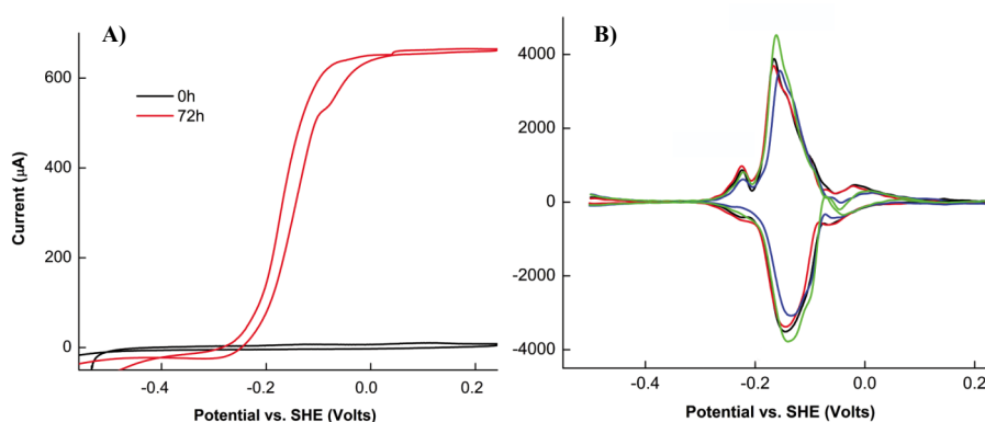
Figure 2. A) Cyclic Voltammetry (1 mV/s) of a Geobacter sulfurreducens biofilm after 72 h growth at +0.2 V vs. SHE on a 2.5 cm 2 planar graphite electrode. B) First derivative analysis of four replicate electrodes, revealing midpoint potentials within the catalytic wave.
